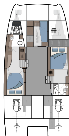
STANDARD 2-CABIN + UTILITY CABIN
